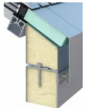
Installation on steel sheet upstand
